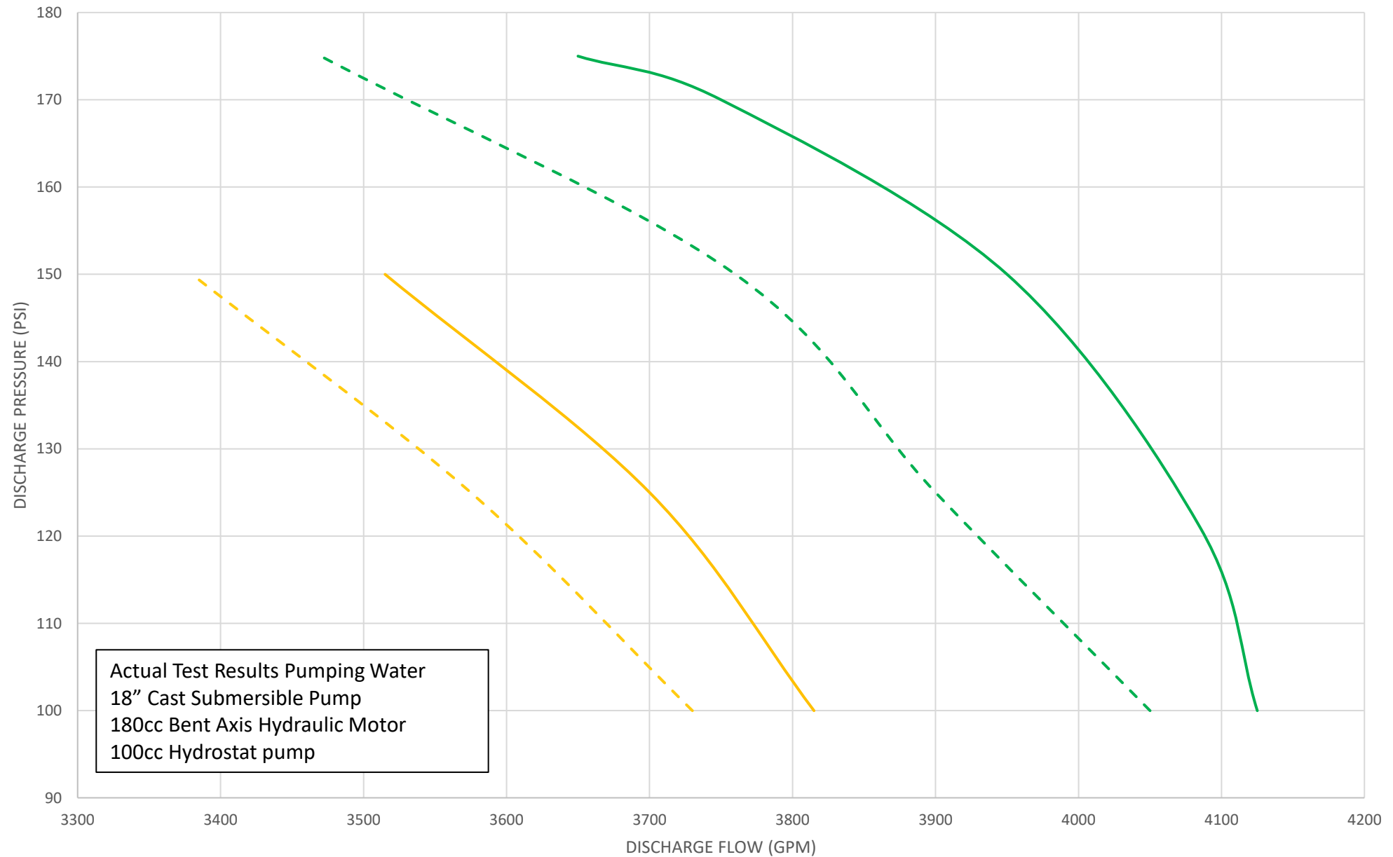
Pump Curve - 18" Cast, Curved 6 Vane, 6819MPC
